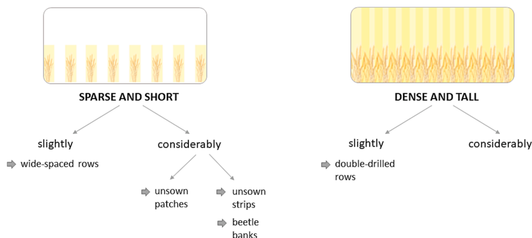
Fig. 1. Classification of measures according to whether and to what extent they aim to make vegetation sparser and shorter or denser and tall. Measures intended to create either a sparse and short or dense and tall crop architecture are listed under each category. The extent is differentiated into slight and considerable (for ‘dense and tall’, no measure with considerable modification is known).
